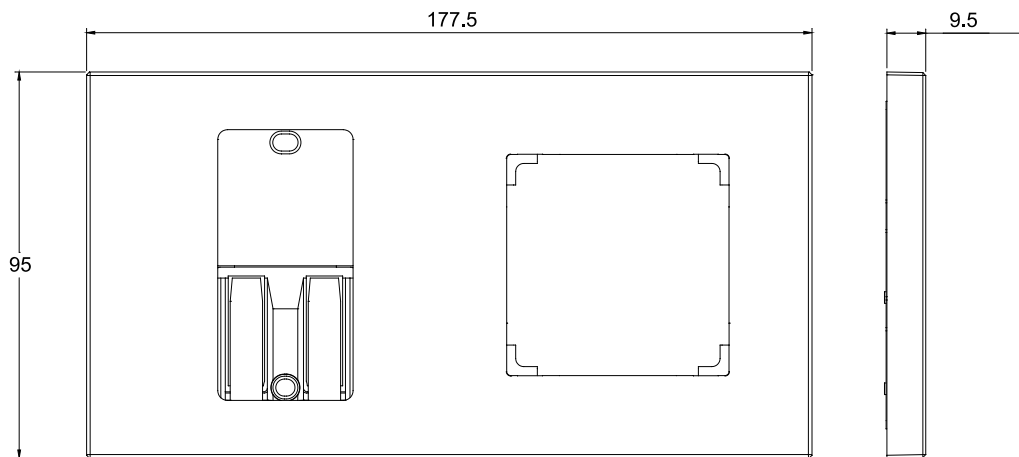
Frame Dimensions
